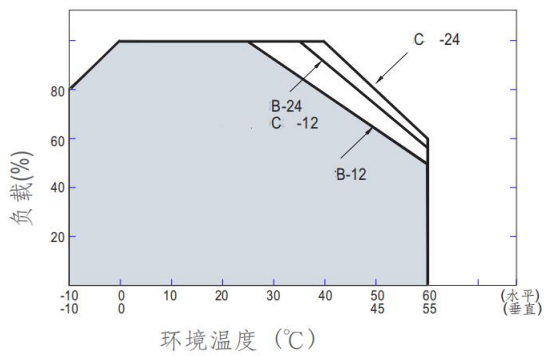
降额曲线:
